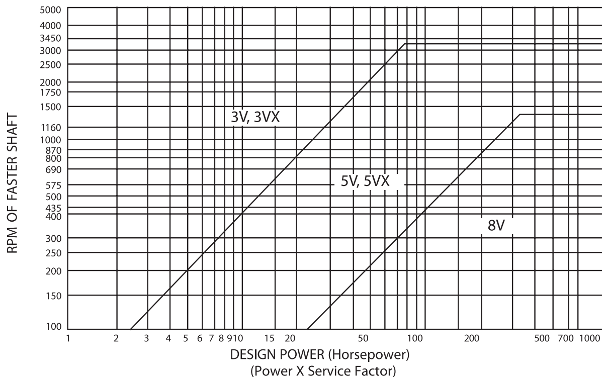
FIGURE 2: NARROW V-BELTS
