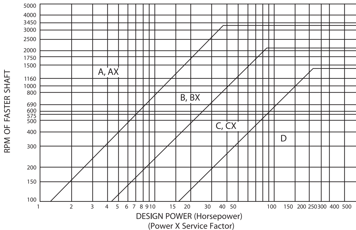
FIGURE 1: CLASSICAL V-BELTS
